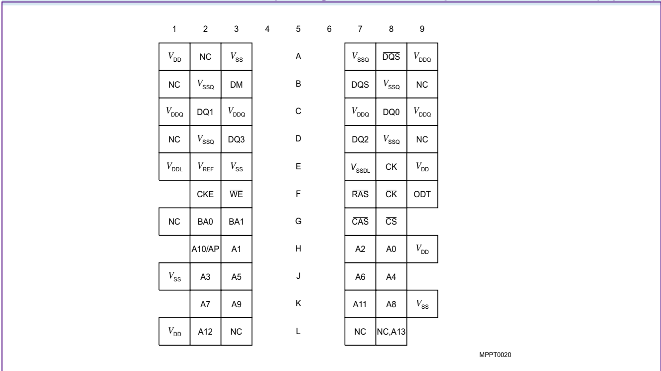
FIGURE 1 Chip Configuration for ×4 components, PG-TFBGA-60 (top view)
